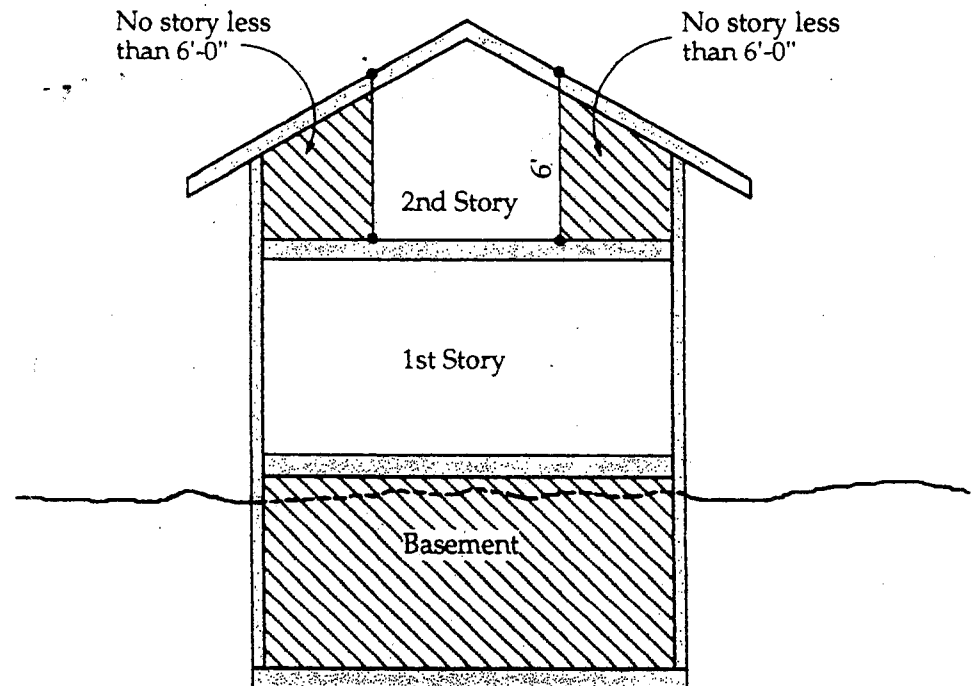
Hatched area represents basement. Over 1/2 its height is below grade. Basement is not considered a story because finished floor above is not 6' above grade.
