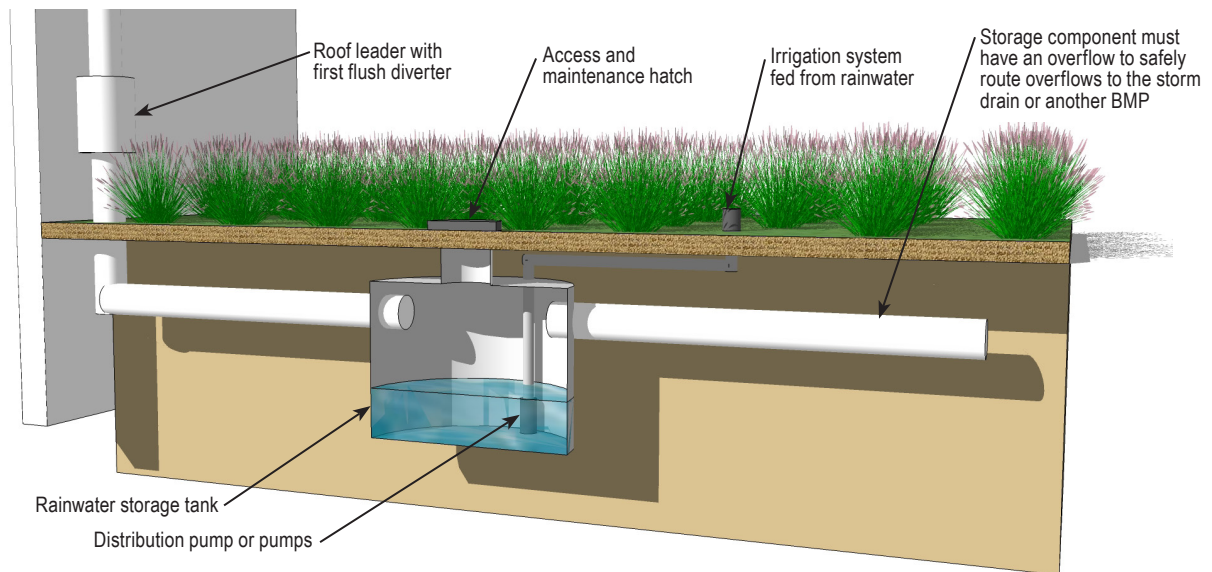
Figure: Rainwater harvesting system typical detail
