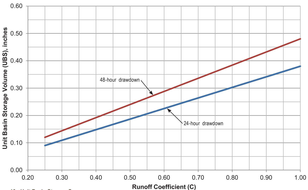
Figure 10: Unit Basin Storage Curves
