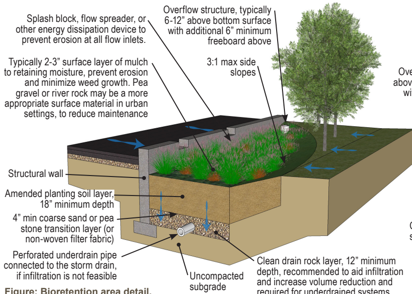
Figure: Bioretention area detail, showing hard edge and soft edge
