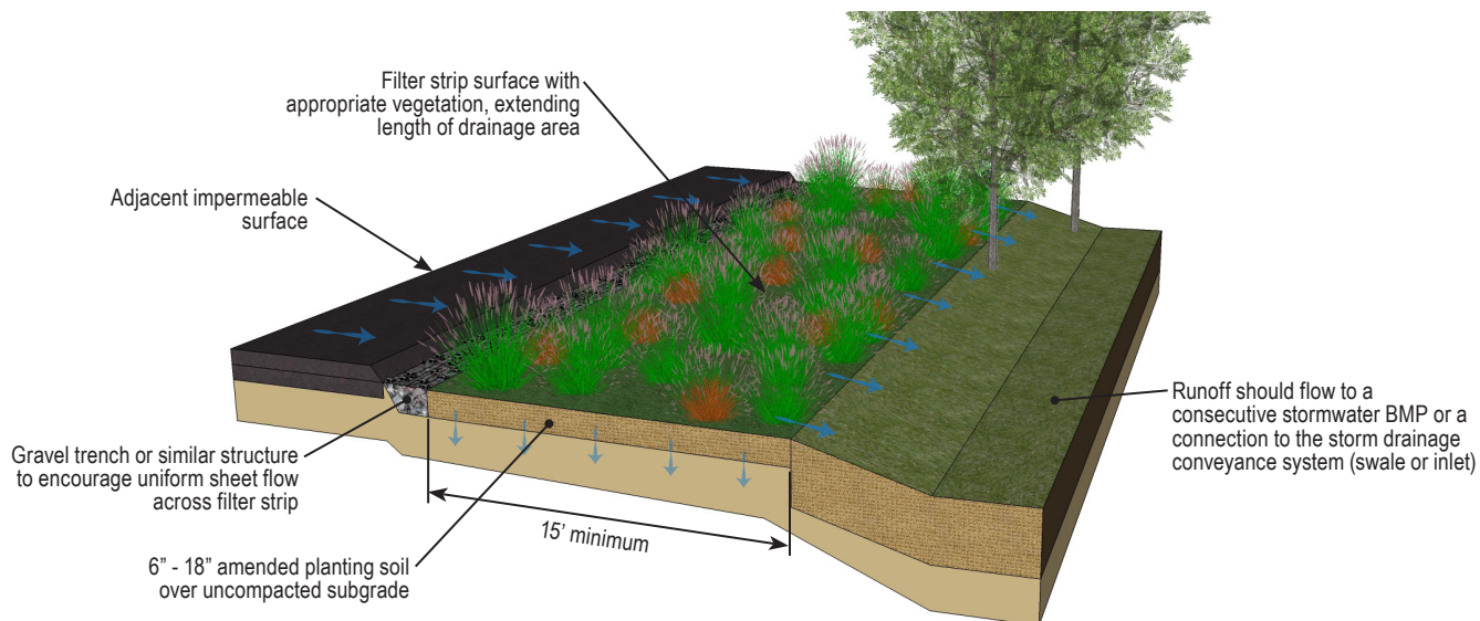
Figure: Filter strip typical detail
