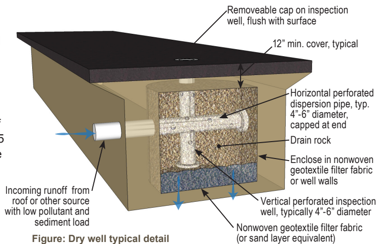
Figure: Dry well typical detail
