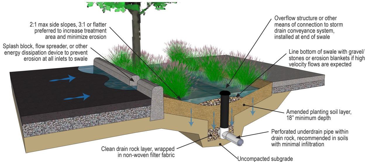
Figure: Vegetated swale typical detail
