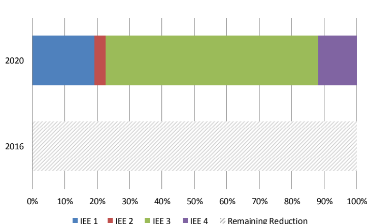
Figure III-9: IEE Emissions Reduction Progress through 2016
