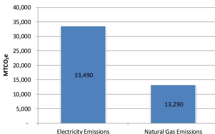
Figure III-10: 2007 Industrial Energy GHG Emissions by Source
