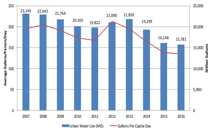
Figure III-18: Urban Water Usage County-wide, 2007-2016
