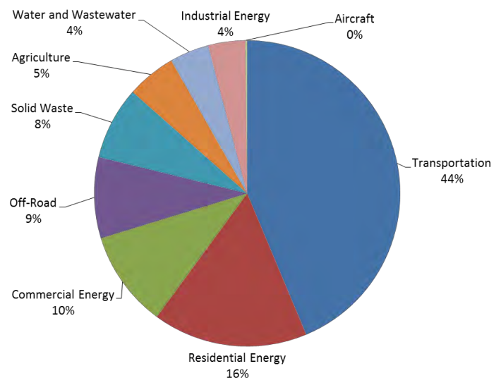
Figure ES-1. 2007 Baseline GHG Emissions by Source (%)
