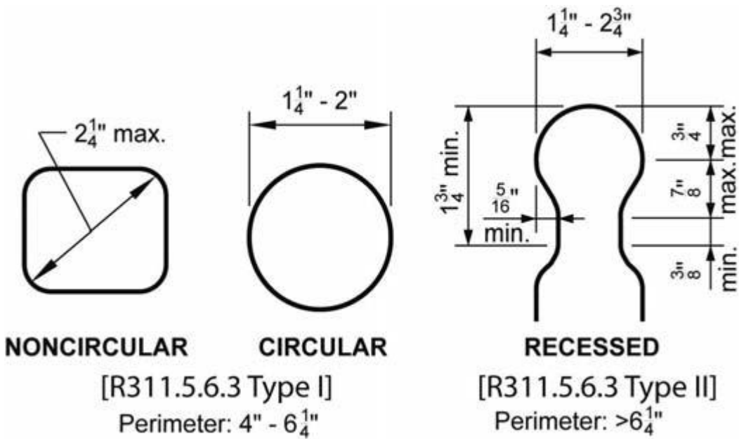
Figure 32B: Handrail Grip Size
