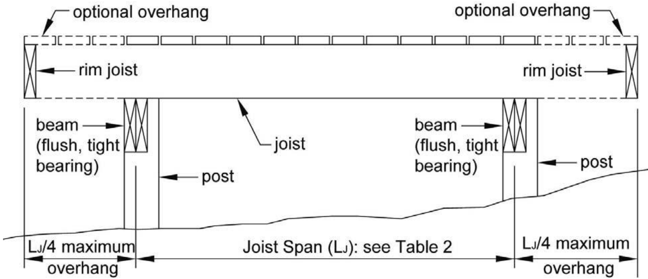
Figure 2: Joist Span – Free Standing Deck
