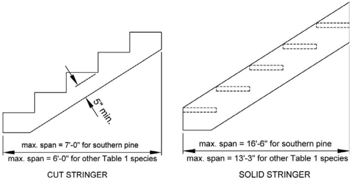
Figure 28: Stair Stringer Requirements
