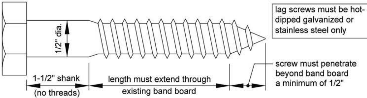
Figure 20: Lag Screw Requirements
