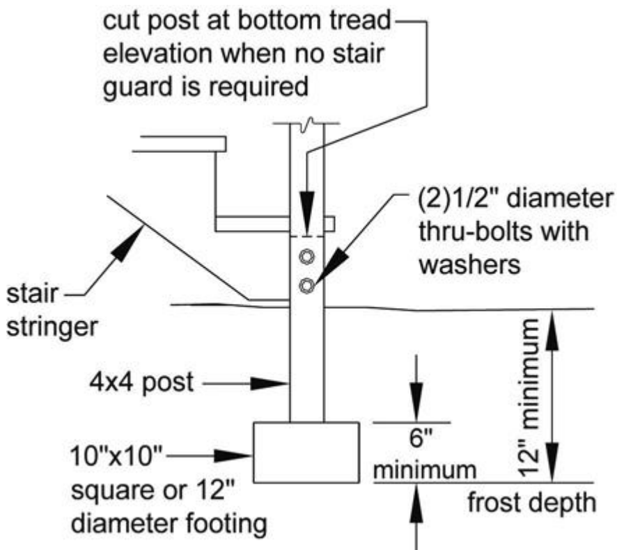
Figure 34: Stair Footing Detail
