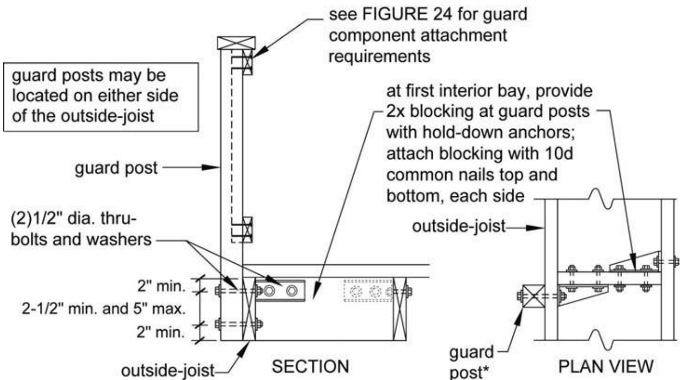
Figure 25: Guard Post to Outside Joist Example
