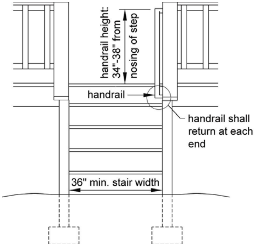
Figure 33: Miscellaneous Stair Requirements
