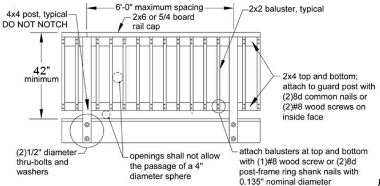
Figure 24: Example Guard Detail
