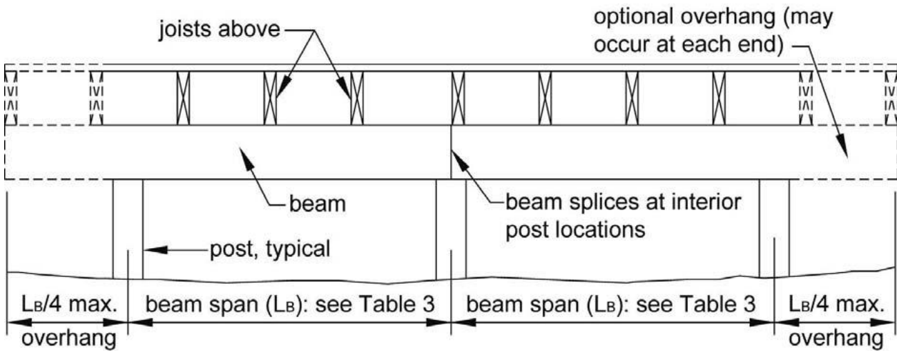
Figure 3: Beam Span Types
