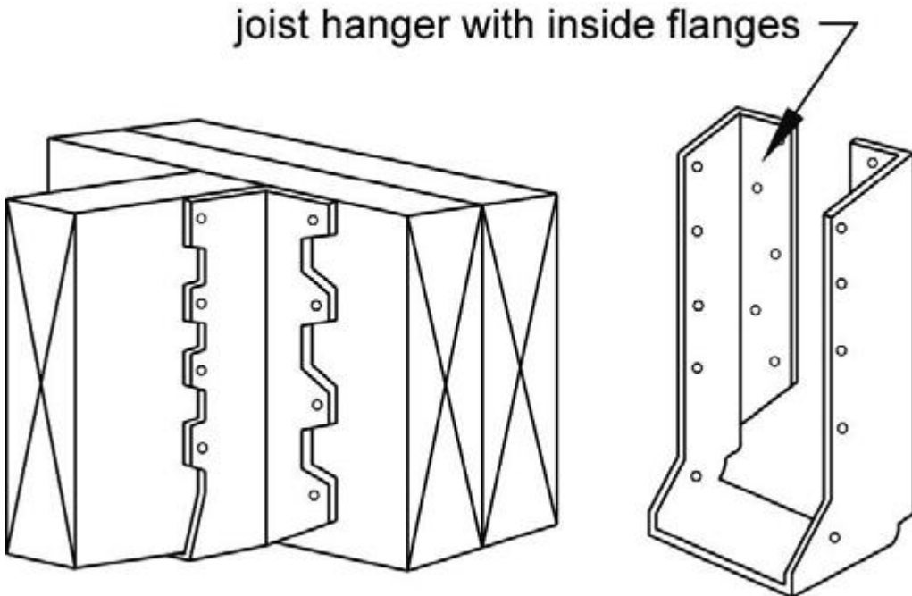
Figure 7: Typical Joist Hangers
