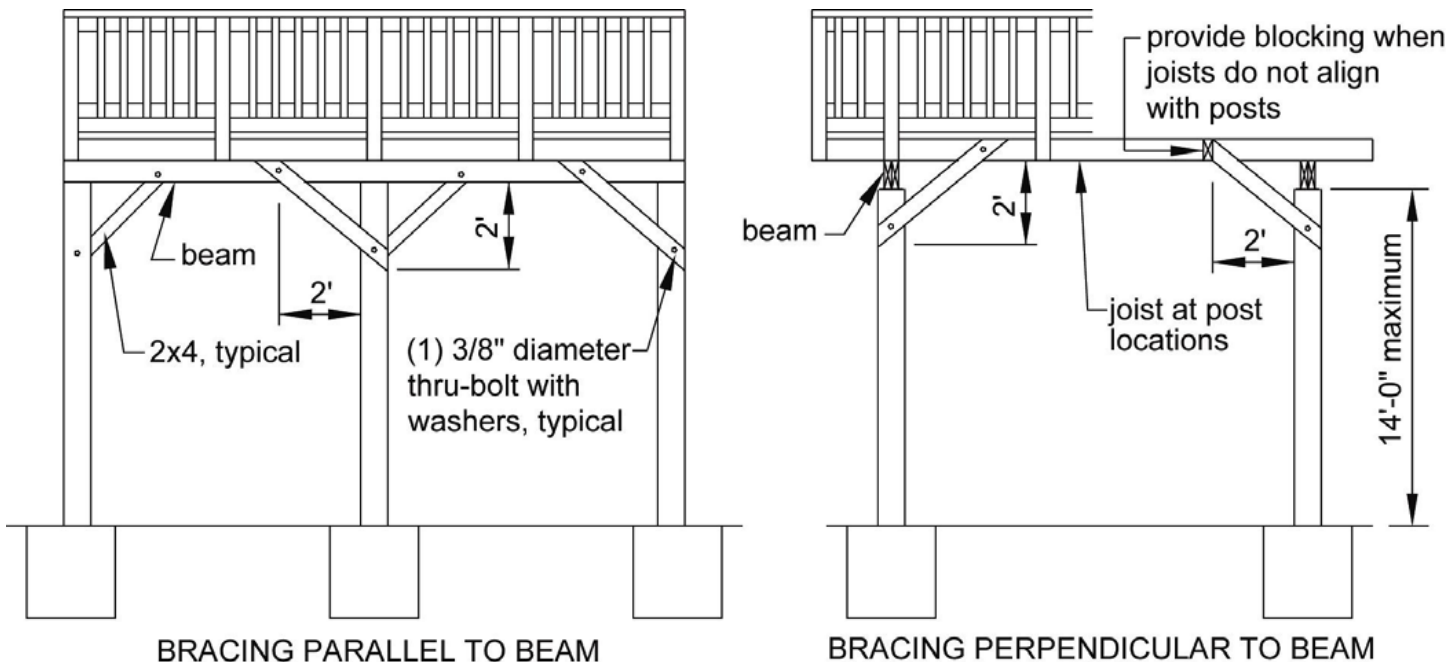
Figure 22: Diagonal Bracing Requirements
