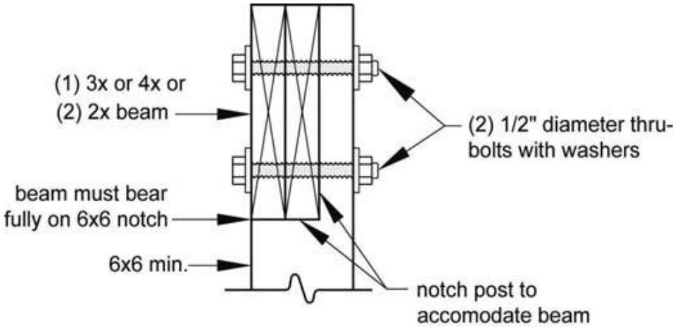
Figure 8: Post-to-Beam Attachment Requirements
