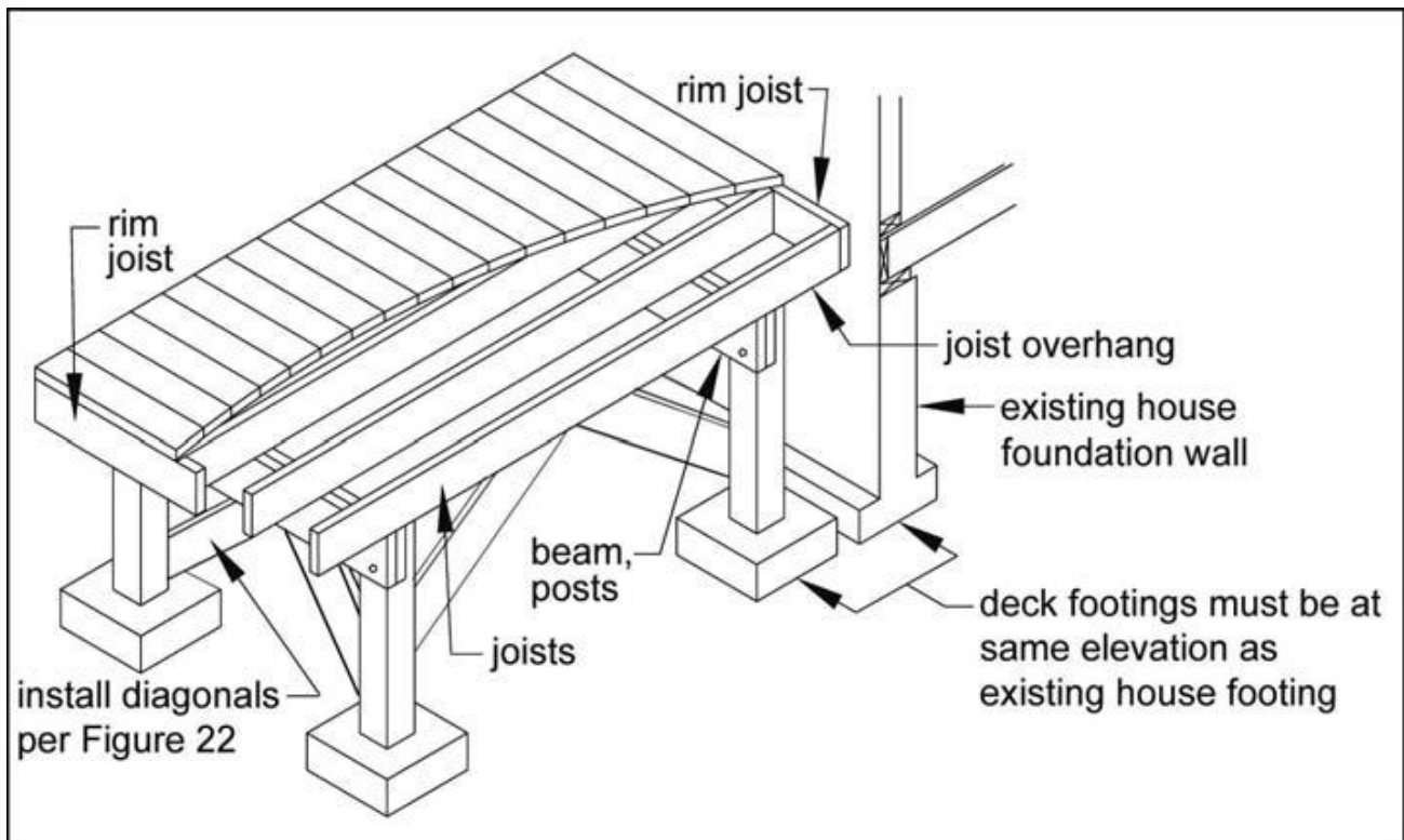
Figure 21: Free-Standing Deck
