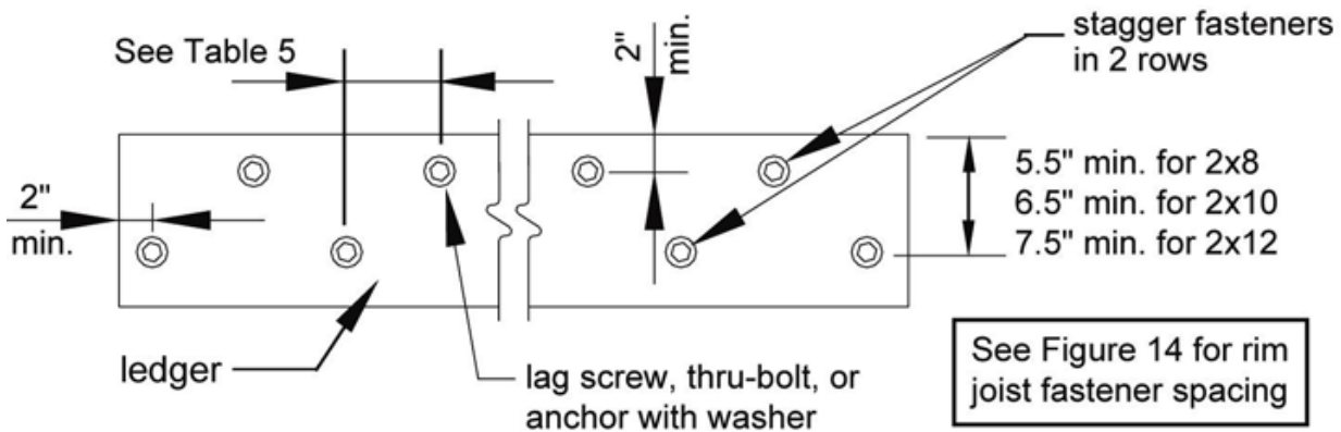
Figure 19: Ledger Board Fastener Spacing and Clearances
