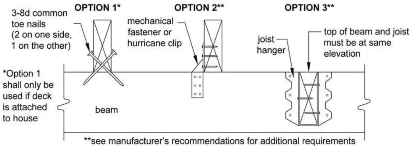
Figure 6: Joist-to-Beam Detail
