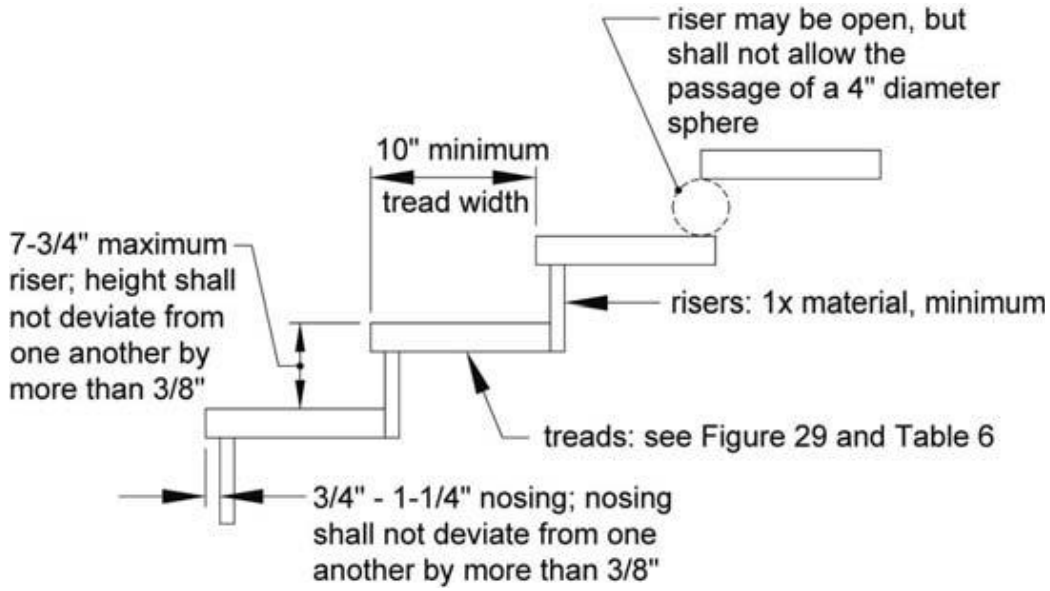
Figure 27: Tread and Riser Detail
